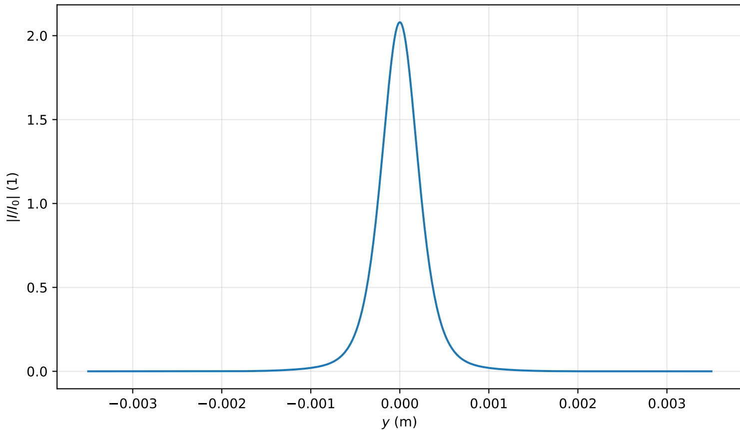
Intensity profile I(x=0, y, z=1.911)/I_0 , \text{Pin}=1.0\text{Pcr} , artificial time
